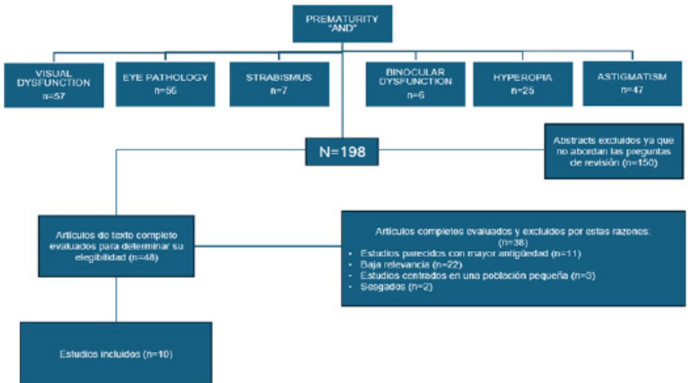
Figura 4. Flowchart
